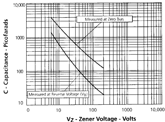
FIGURE 4 Typical Capacitance Vs. Zener Voltage
